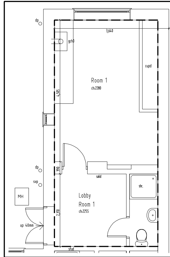
ROOM 1 PLAN
