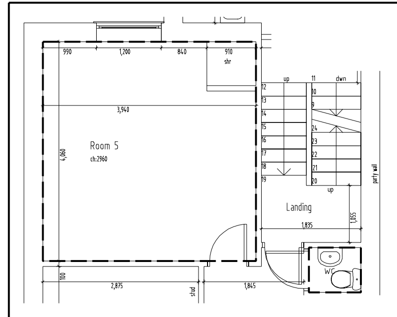
ROOM 5 PLAN
